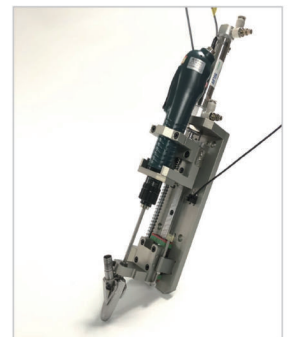
Screwdriver for using with automation
