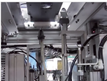
Fastening screws from bottom side
